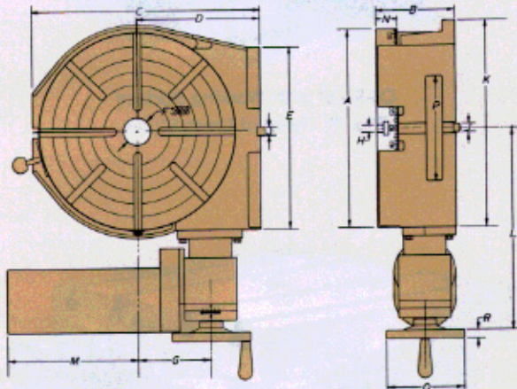
OUTLINE MODELS U-12-P; U-15-P; U-20-P; U-25-P; U-30-P.
