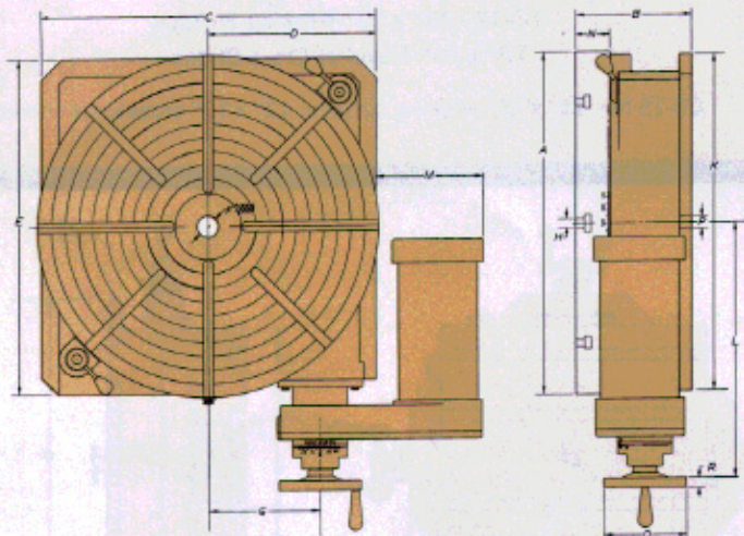
OUTLINE MODEL P-25
