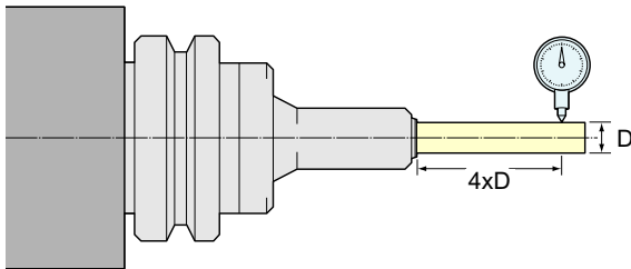
Excellent run-out accuracy ( 3\mu\text{m} at 4xD )
