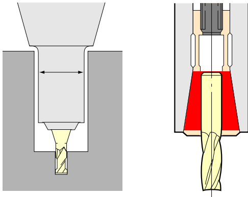
Slim and compact nose with strong gripping
